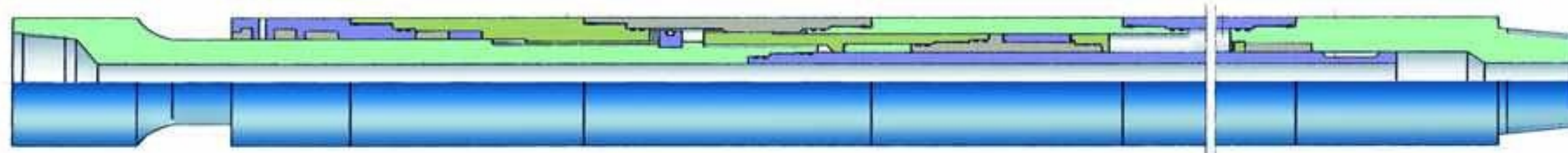
SJ型双向减震器 SJ Double-Way Shock Absorber
