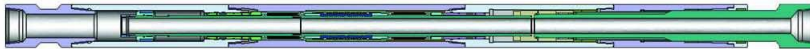
QJZ型全机械式震击器 QJZ Mechanical Drilling Jar
