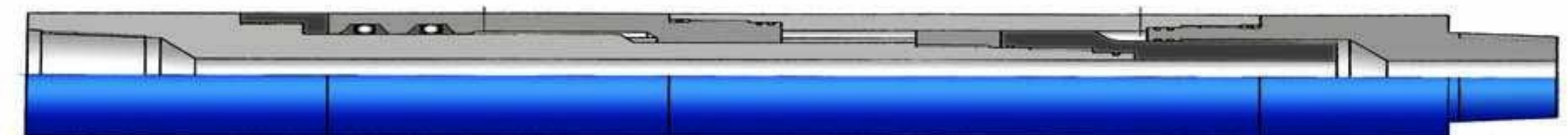
BXJ型封闭式下击器 BXJ Type Lubricated Fishing Bumper Sub
